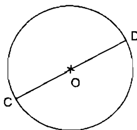
b) \alpha = 180^\circ
